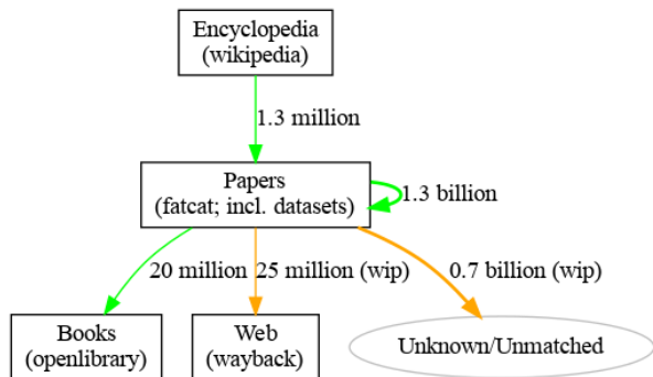
Figure 1: Schematics of the main reference entities; green: included in the corpus; orange: currently in development; gray: Planned, but not in development; red: long-term desiderata.
